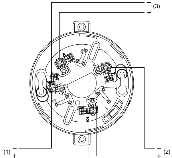
Figure 1: Typical base wiring
